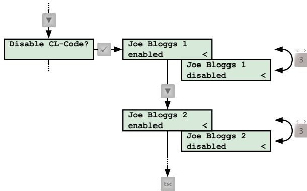
Menu item "Disable comlock/cryplock code"
