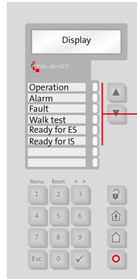
Keypad LED indication
