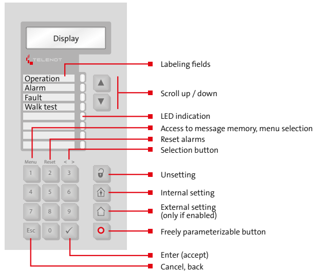
Structure of BT 820
